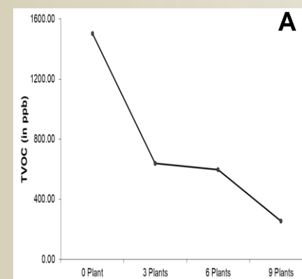
Fig. A. Reduction in TVOC concentrations indoors by Areca Palm
